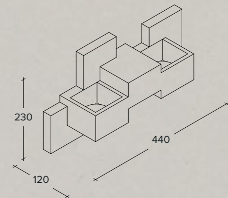
Three-lights Up/down plaster wall lamp (Modello depositato)
