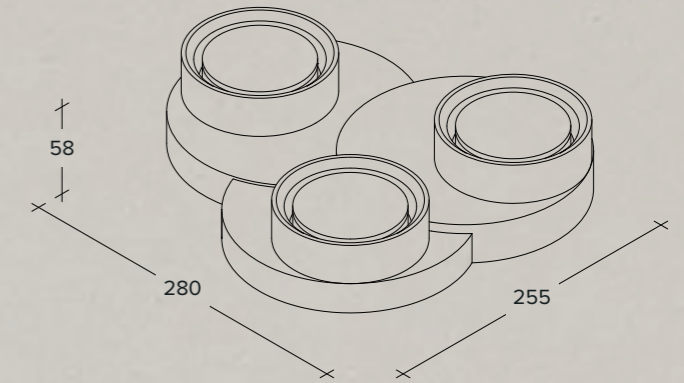
Three-lights plaster ceiling lamp (Modello depositato)
