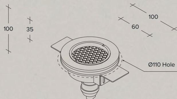
Recessed plaster spotlight with matte black painted ring and mesh finishing
