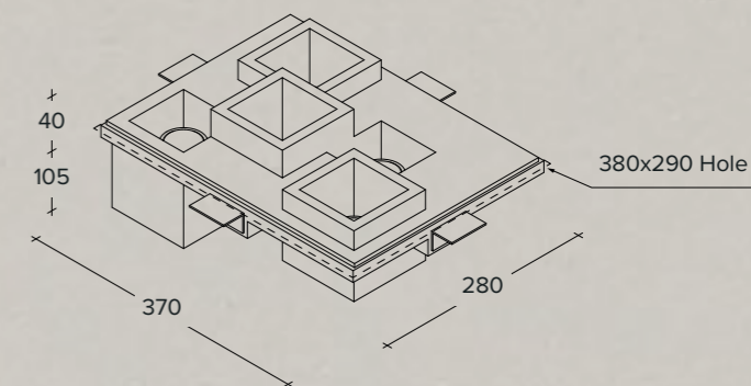
Five-lights recessed plaster spotlight
