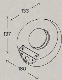
Plaster wall lamp for indirect lighting (Modello depositato)
