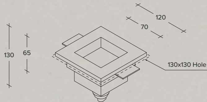
Invisible recessed fitting for false ceilings
