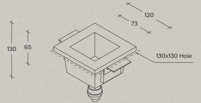
Recessed plaster spotlight with adjustable light point
