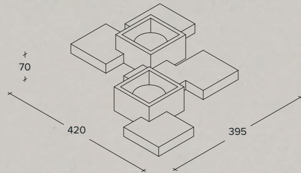
Two-lights plaster ceiling lamp (Modello depositato)
