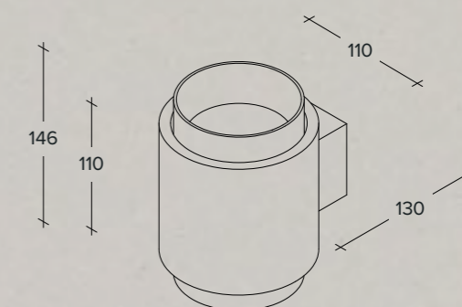
Plaster wall lamp for indirect lighting with aluminium ring in different finishings
