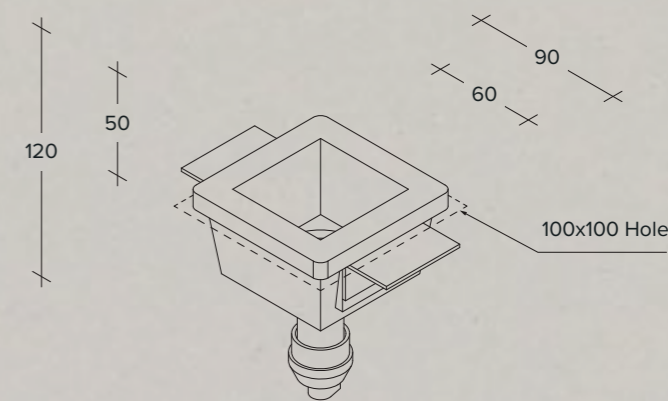
Recessed plaster spotlight
