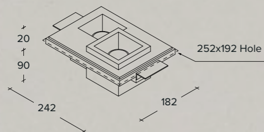
Two-lights recessed plaster spotlight
