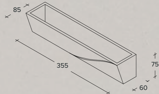
Two-lights dual emission plaster wall lamp with frontal beamline
