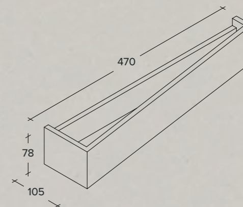
Plaster wall light, dual emission
