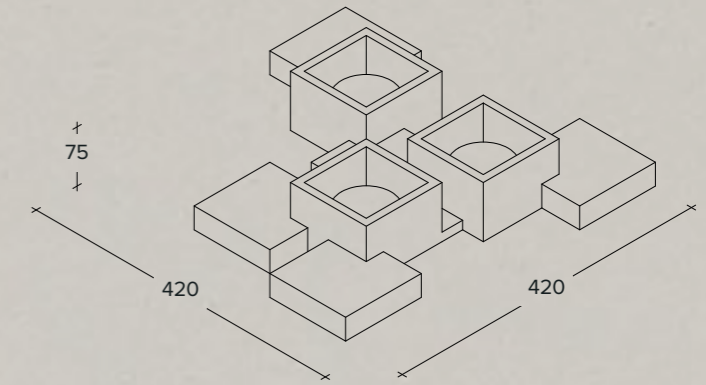
Three-lights plaster ceiling lamp (Modello depositato)
