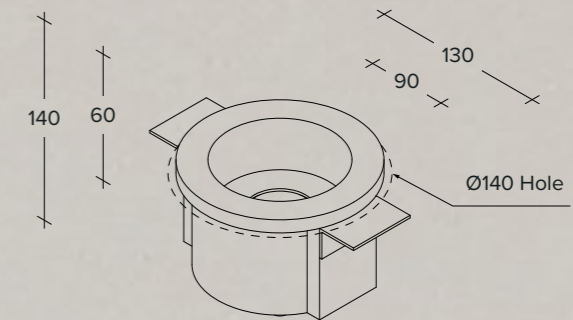
Recessed plaster spotlight. Internal metal housing with IP44 protection rating
