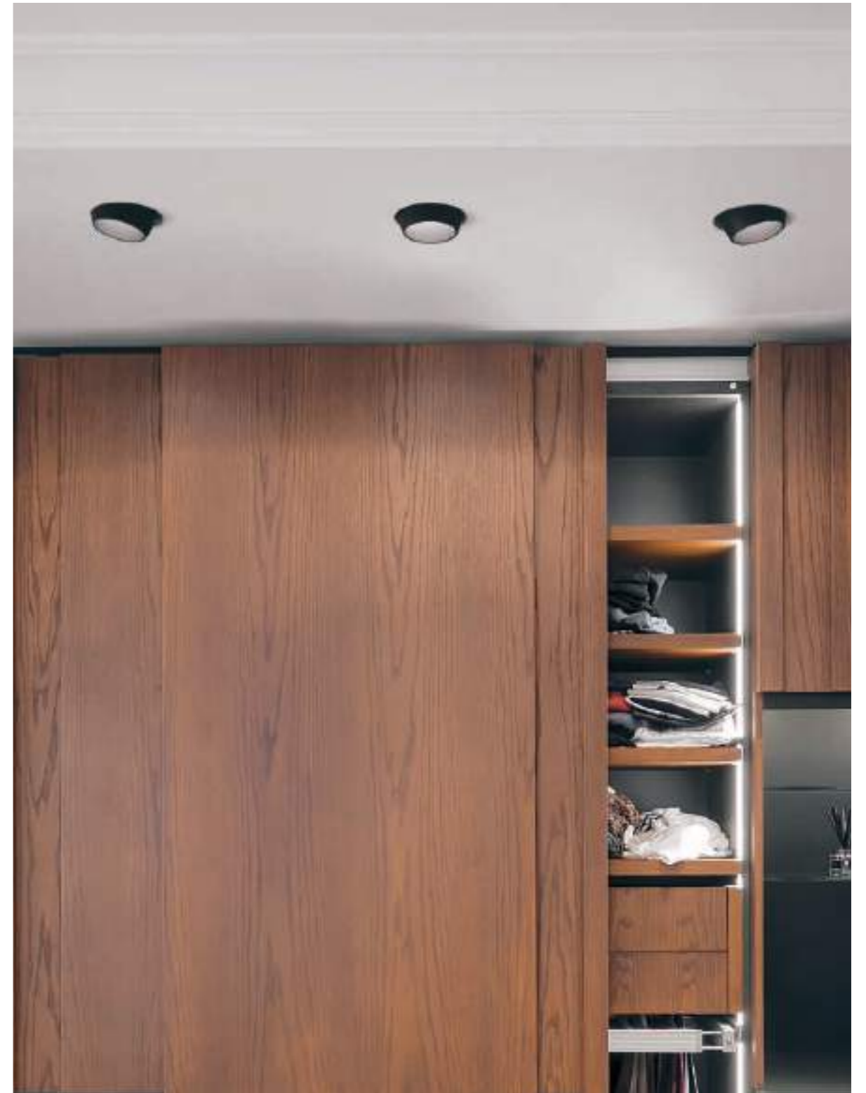
←↓ T356 Lelanto One-light adjustable recessed plasterboard spotlight with matte black painted ring finishing. Adjustable 15° tilt light. GU10 - 1x40W Ø50 mm aluminium ring
