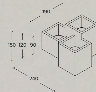
Three-lights plaster ceiling lamp
